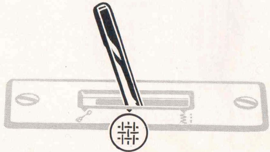
Throat plate raised for darning, embroidery and button sewing.
